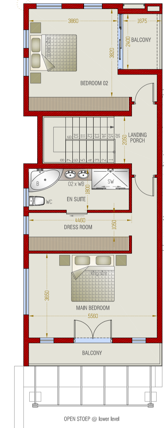
PROPOSED FIRST STOREY PLAN SCALE 1:100
