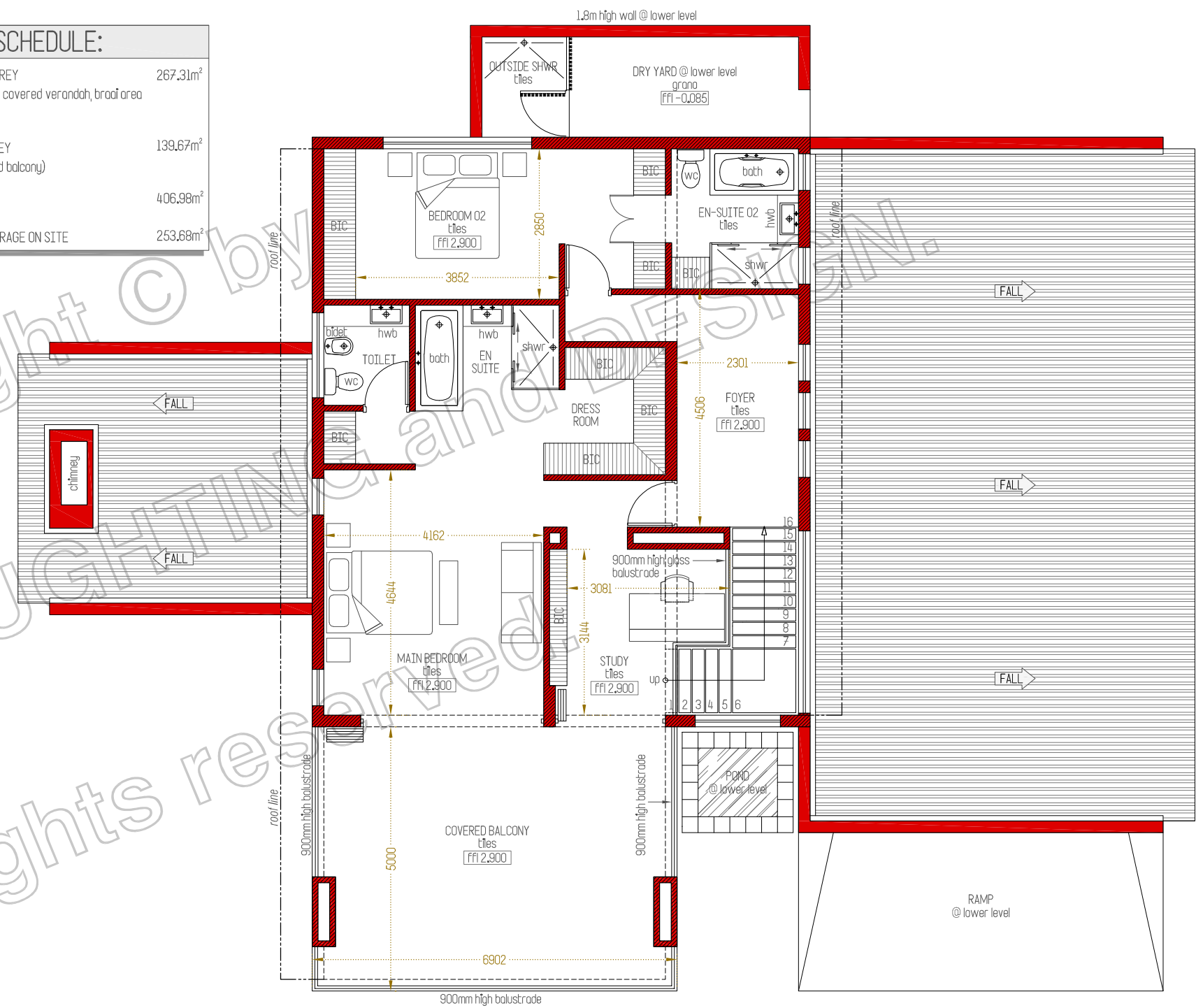
FIRST STOREY PLAN
